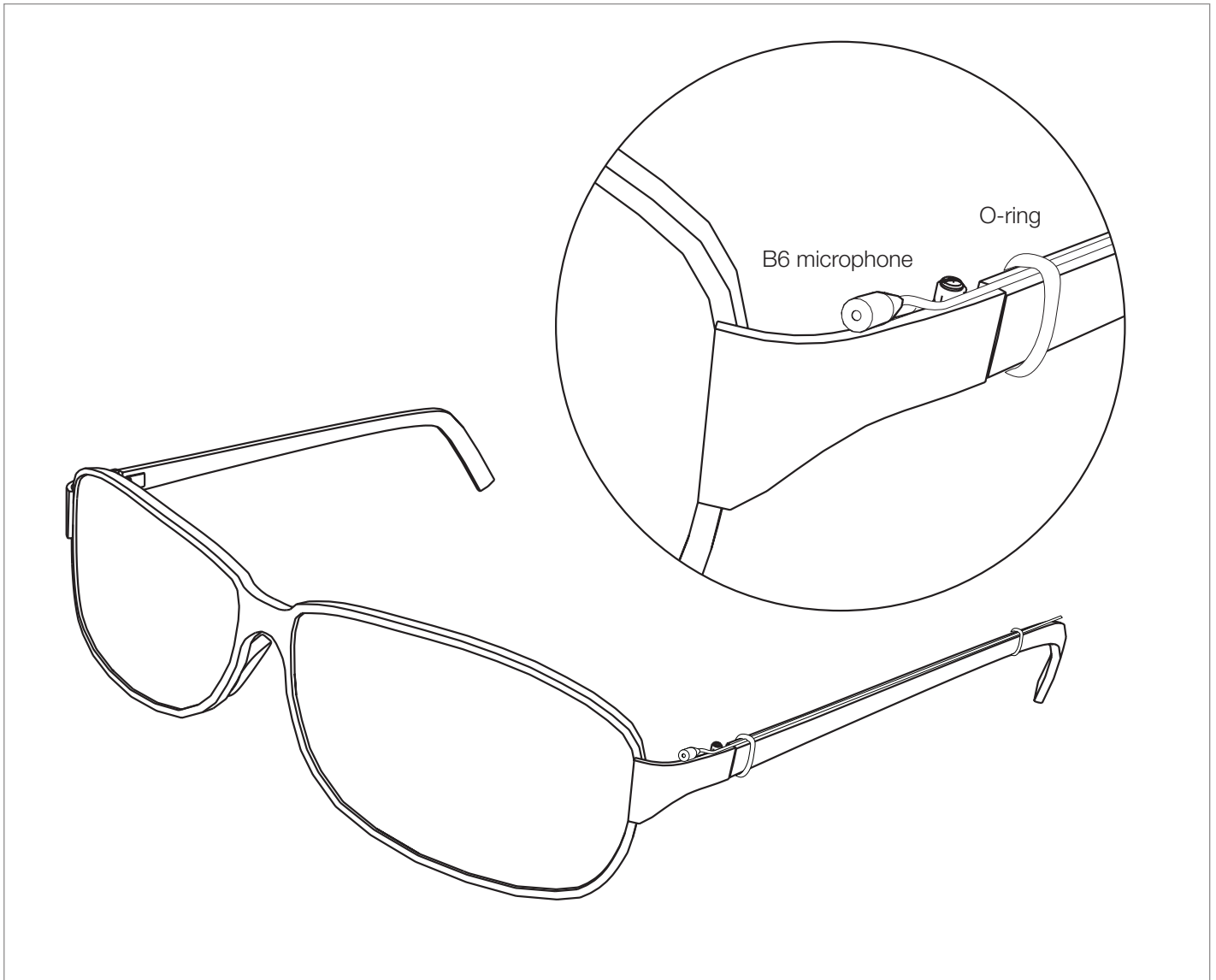
Figure 1: B6 lavalier microphone attached to a pair of eyeglasses.
